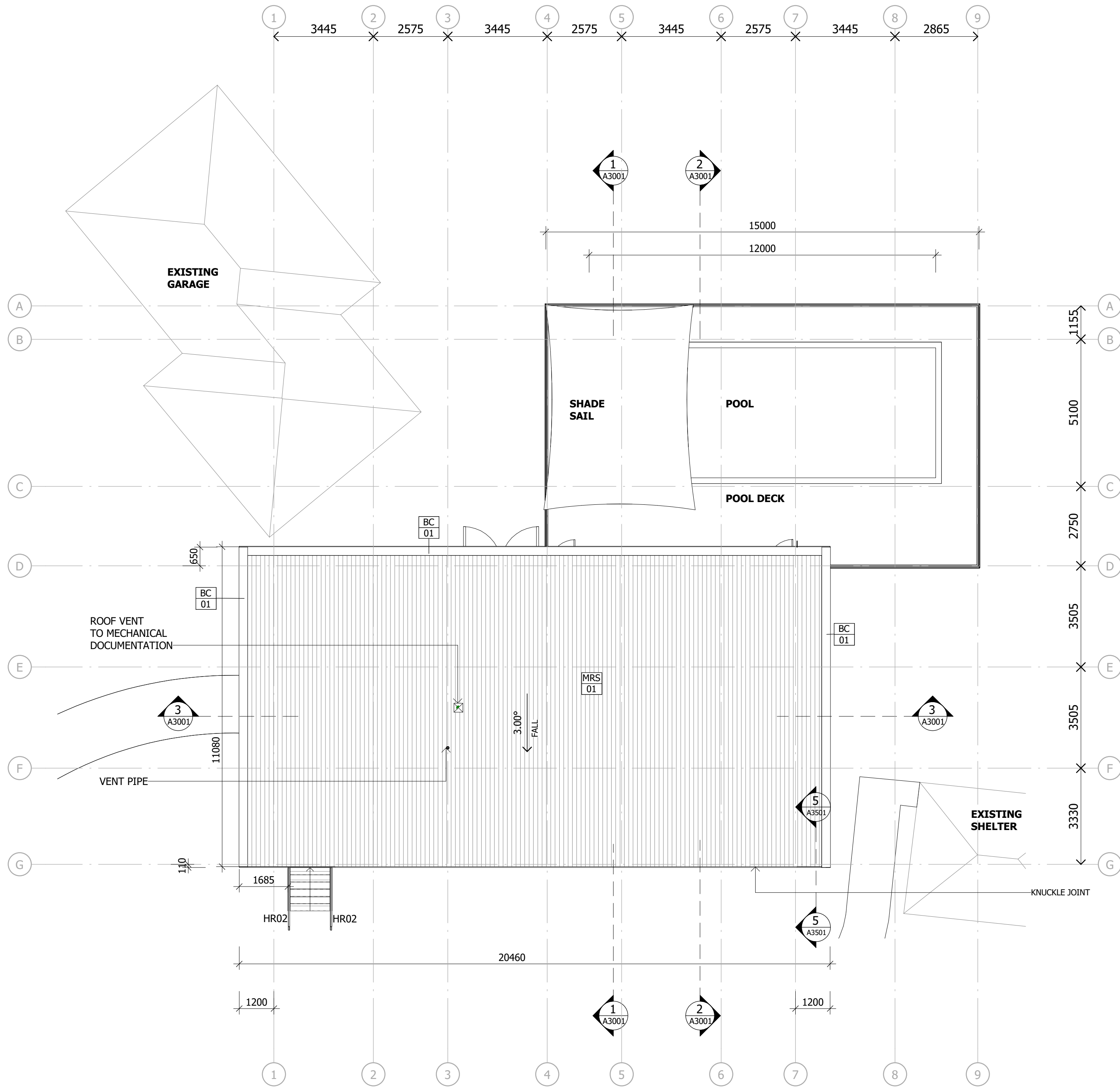
1 GA PLAN - ROOF A2001 1 : 100
